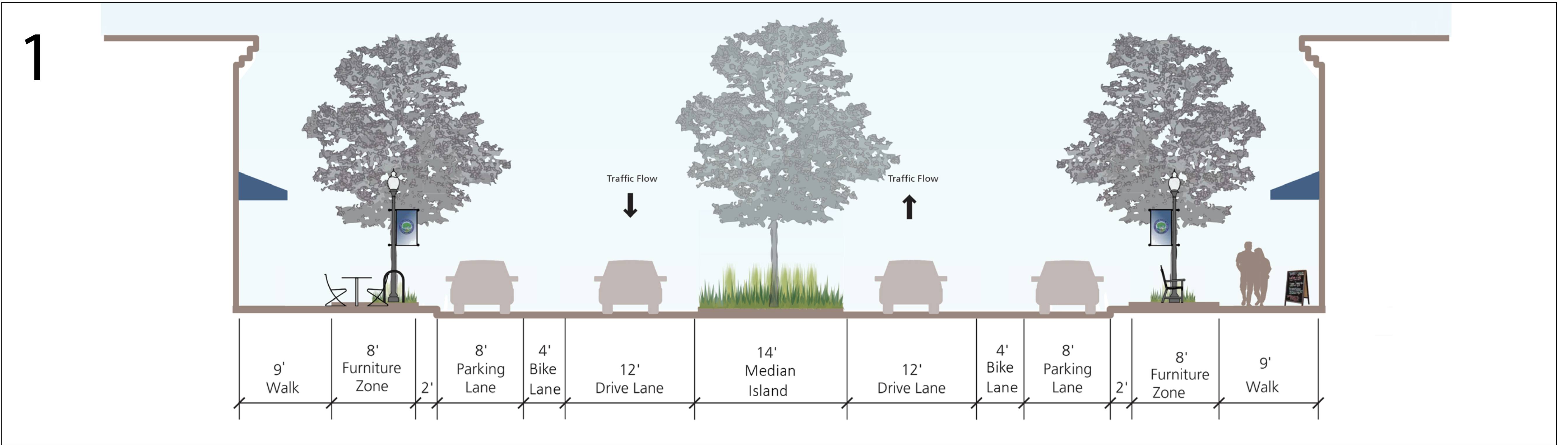
COCHRAN AVENUE (M-50) AT MEDIAN
